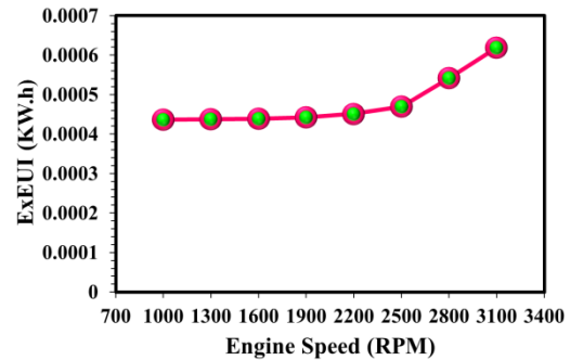
Figure 20: ExEUI at various engine speeds.
